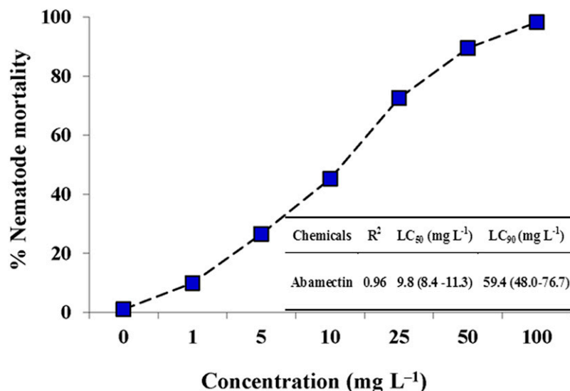
Fig. 1. Nematode mortality (%) and lethal concentrations (LC 50 and LC 90 ) (mg liter -1 ) of abamectin against Heterodera avenae juveniles (J2s) when incubated for 24 h at 16°C.
