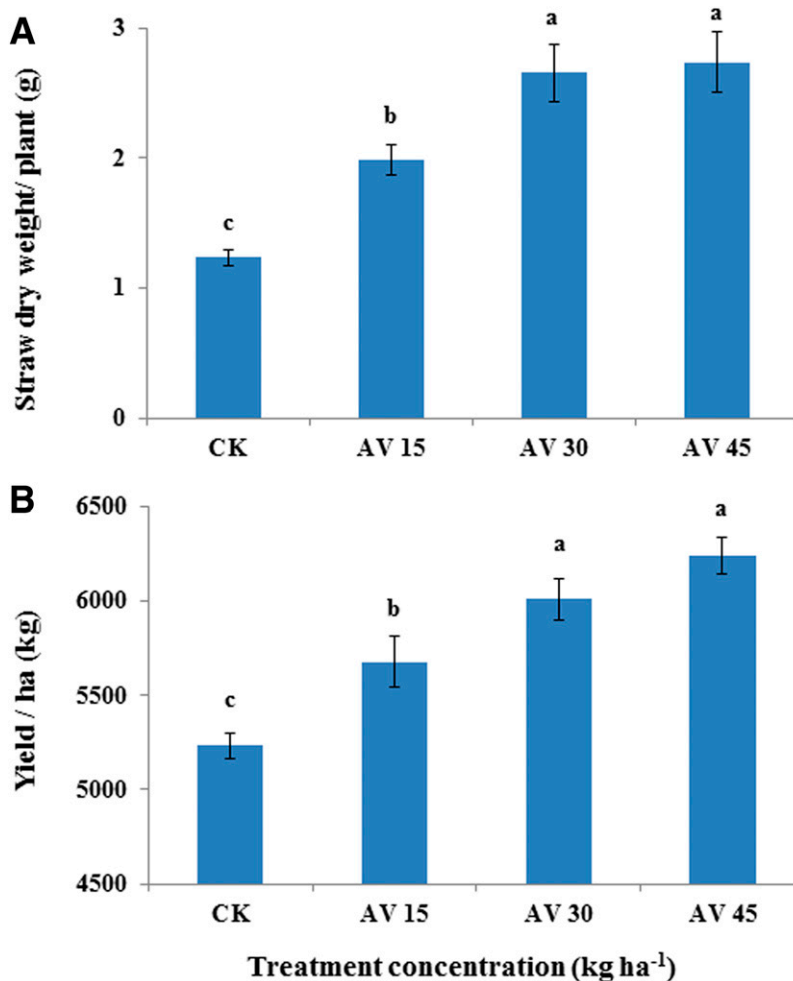
Fig. 2. Influence of abamectin (AV) on wheat plant growth during two years of testing in soils naturally infested with Heterodera avenae . The bars correspond to the standard error. Bars with different letters are significantly different ( P = 0.05 ). A , Influence of abamectin on straw dry weight; B , influence of abamectin on grain yield.
